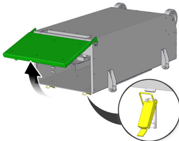
Fig. 4-3: Couvercle
