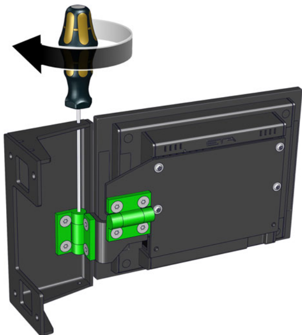
Fig. 2-5: Charnières
