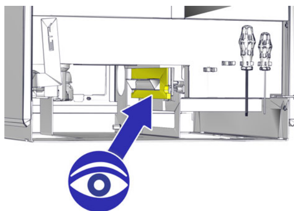
Fig. 4-4: Joint
