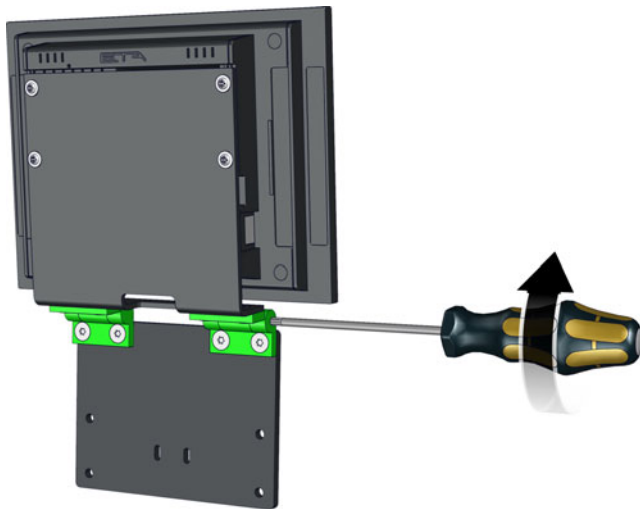
Fig. 2-5: Charnières
