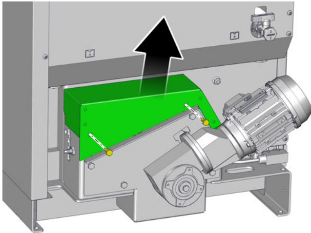
Fig. 8-20: Cache
