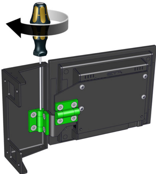
Fig. 2-5: Charnières
