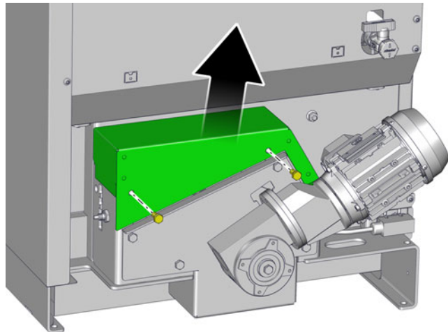
Fig. 8-24: Cache
